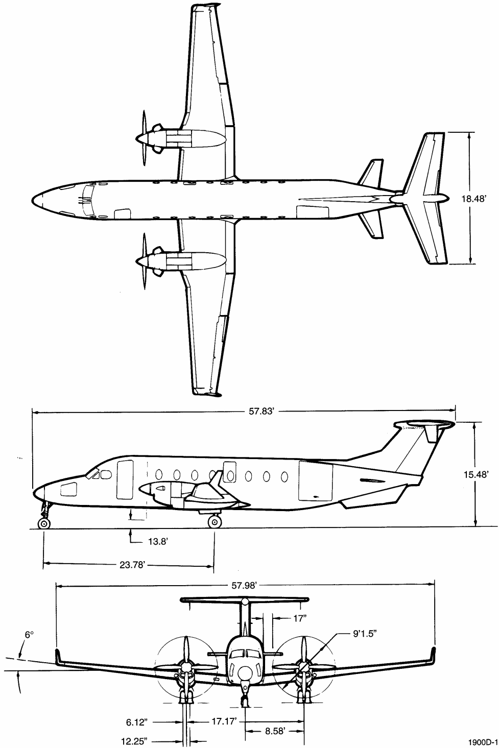
Airplane Dimensions
